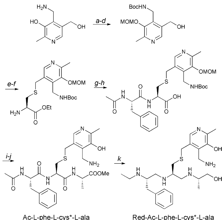
Scheme 4. Reagents and conditions: (a) \text{Boc}_2\text{O} , \text{Et}_3\text{N} , 90%; (b) \text{TBDMSCl} , Im, 95%; (c) \text{MOMCl} , \text{NaH} , 75%; (d) \text{TBAF} , 86%; (e) \text{MsCl} , \text{Et}_3\text{N} , quantitative; (f) \text{L-Cys-OEt} , \text{NaH} , 87%; (g) \text{Ac-L-Phe} , \text{HATU} , i\text{-Pr}_2\text{NEt} , 95%; (h) \text{LiOH} , \text{THF} , 70%; (i) \text{L-Ala-OMe} , \text{HATU} , i\text{-Pr}_2\text{NEt} , 82%; (j) \text{TFA} , 95%; (k) \text{BH}_3\cdot\text{THF} , 80%.
