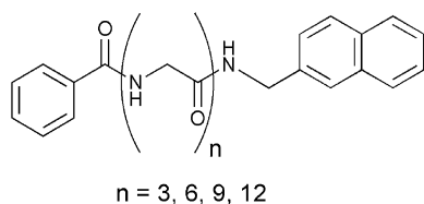
Figure 1. Polyglycine pre-cursors for BH 3 ·THF reduction.
