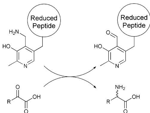
Scheme 3. Proposed pyridoxamine-mediated transamination of α-ketoacids to α-amino acids.
