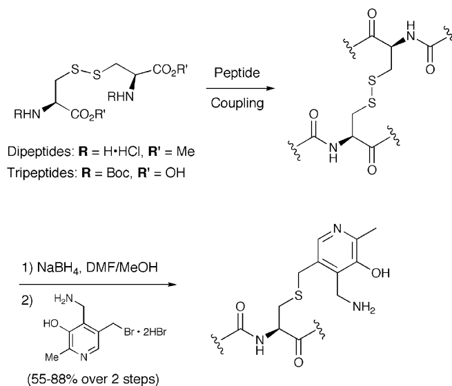
Scheme 5. Alternative route toward pyridoxamine-ligated cysteine containing di- and tripeptides.
